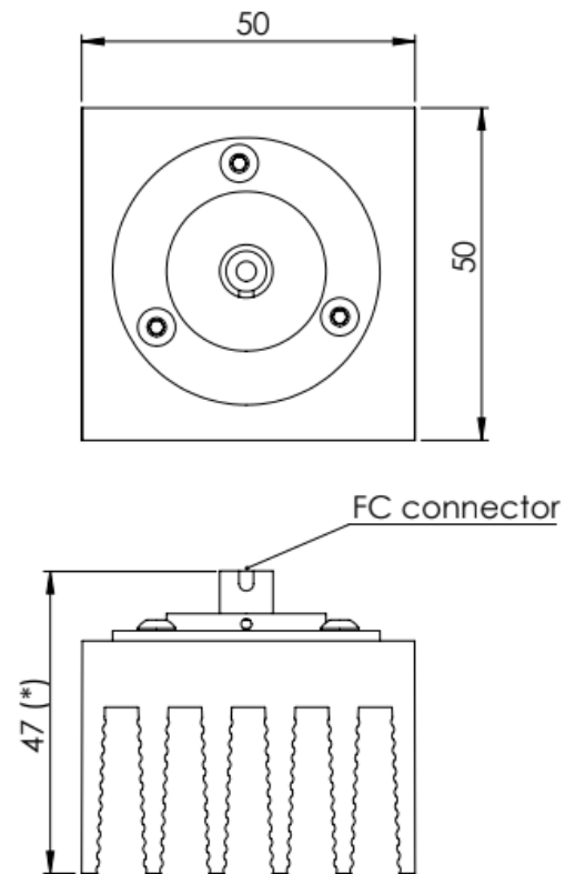
FC connector
