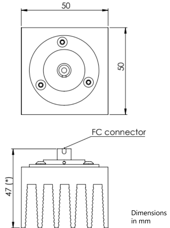
FC connector
