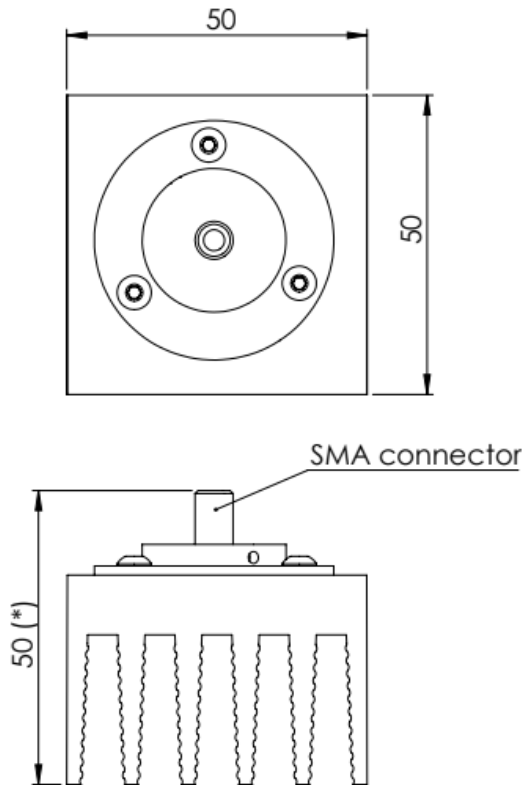
SMA 905 connector
